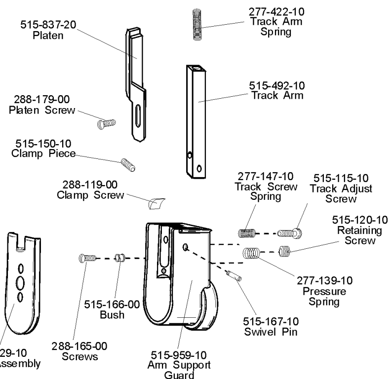
515-766-20 Complete Replacement Arm Attachment
